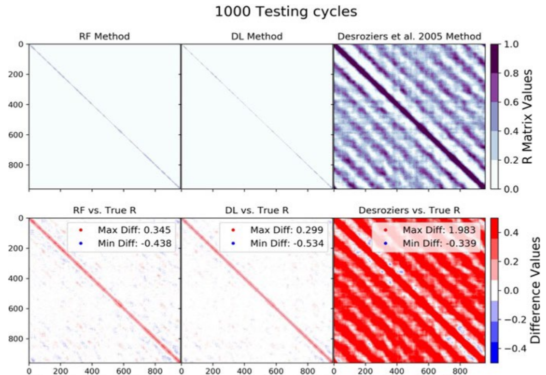
Figure 4: Similar to Figure 3 but predicting the identity \mathbf{R} matrix under changing model forcing conditions.
